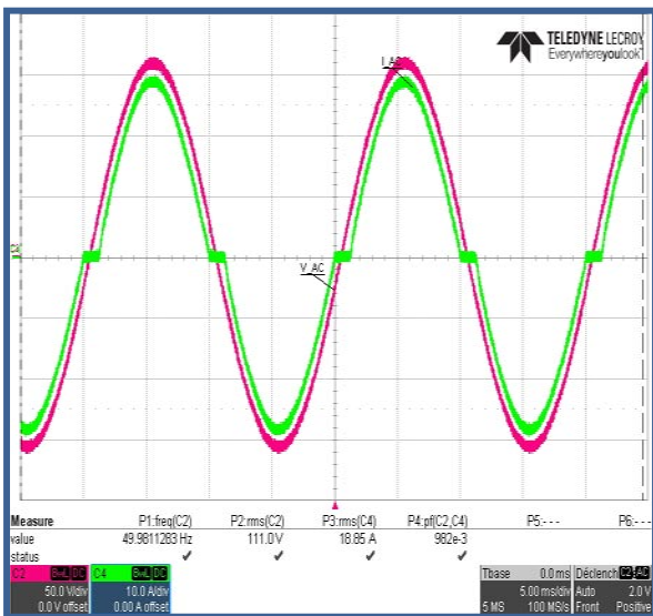
Input Current @ 115Vac 50Hz 2000W
