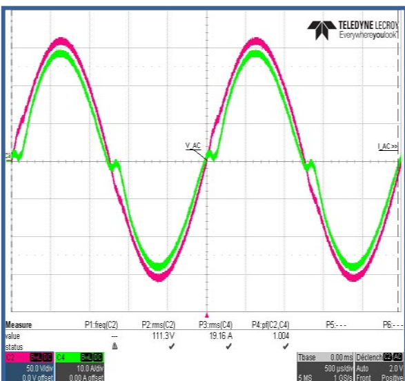
Input Current @ 115Vac 400Hz 2000W
