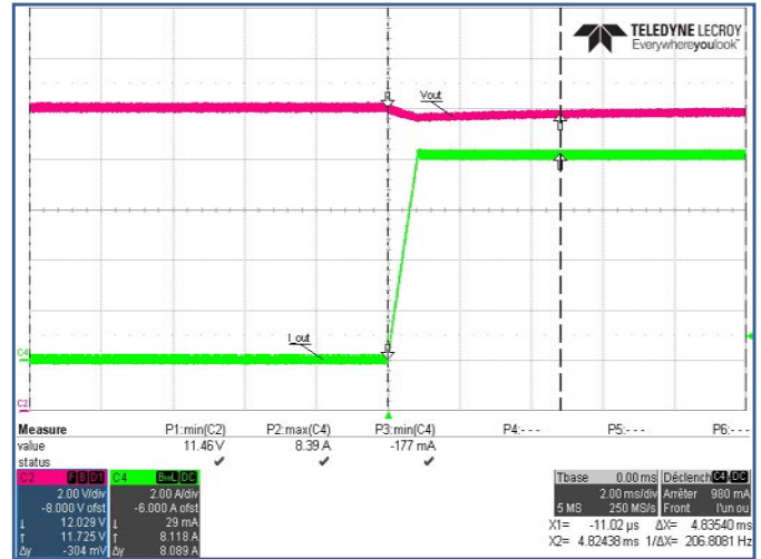
Output voltage Regulation 5V / 150A converterPAC
