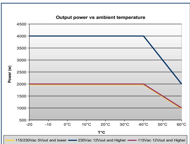
Power vs. Ambient temperature
