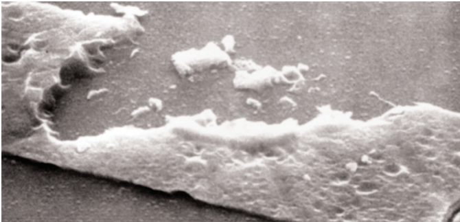
Figure 1. Latent damage due to ESD discharge
