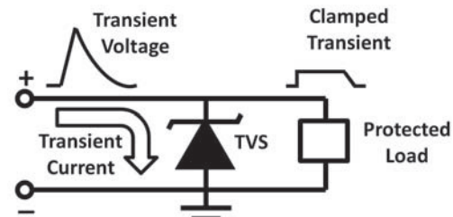
Figure 8 Transient Voltage Suppression operation
