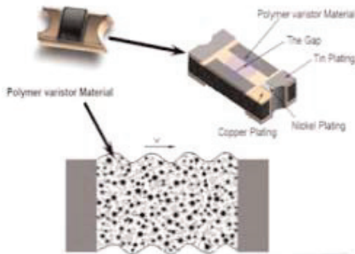
Figure 5. Voltage variable material ESD suppressors
