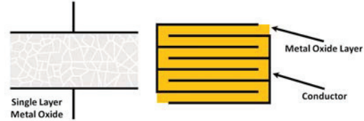
Figure 6 Multilayer varistor construction
