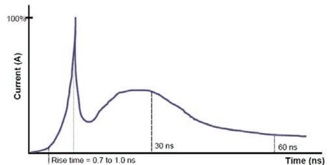
Figure 4. ESD pulse
