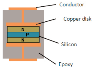
Figure 7. Transient Voltage Suppression construction
