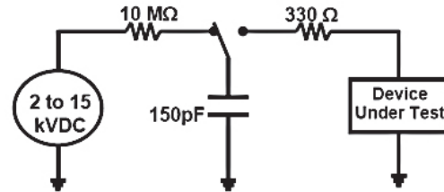
Figure 3. Test setup for Human Body Model
