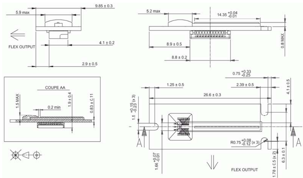
Figure 2 Sensor dimensions
