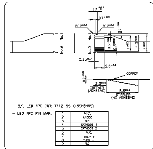
DETAIL "b" (N/S)
