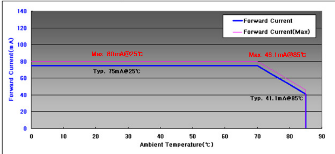
Ambient Temperature vs. Allowable Forward Current
