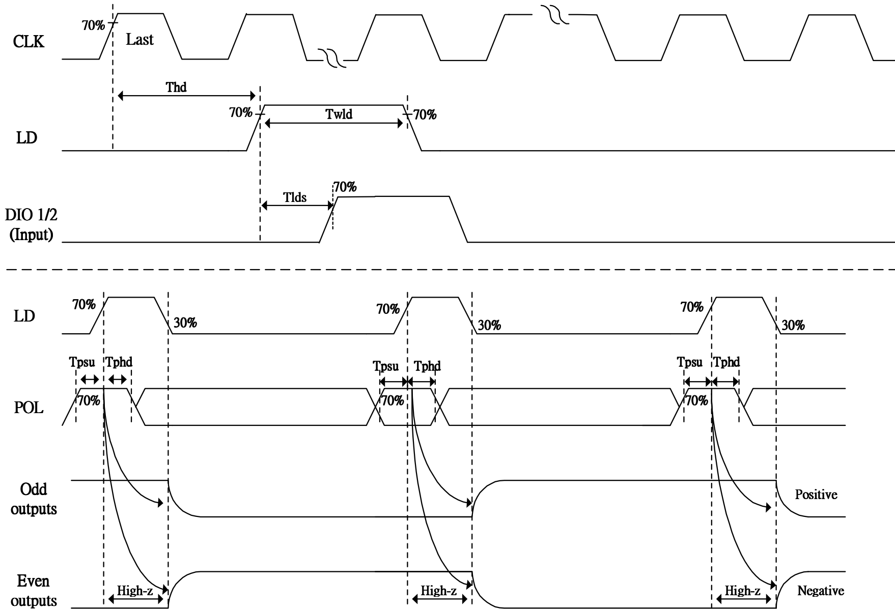
Fig. 11-2 Horizontal timing(2)
