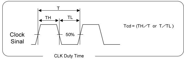
Fig2 Input signal timing \Delta 1
