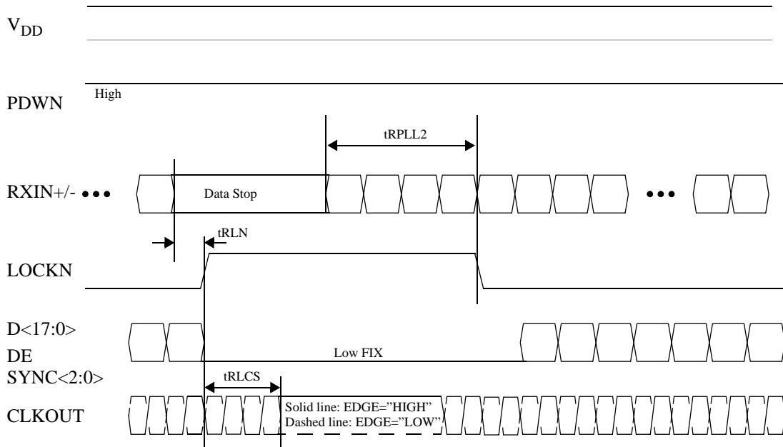
Fig. 10 Receiver Lock Recovery Sequence
